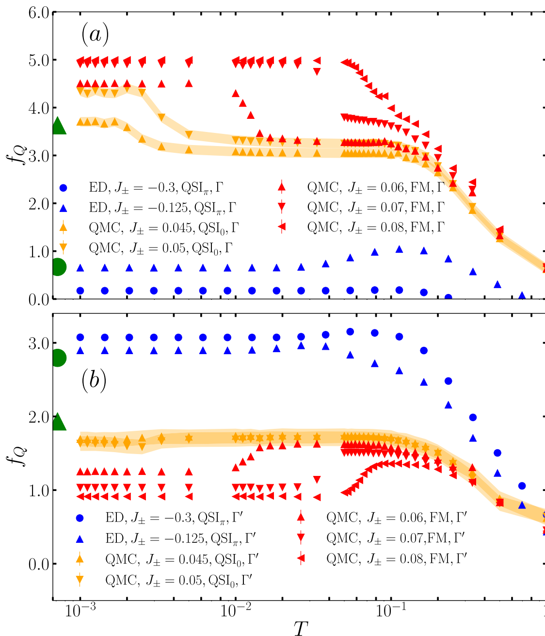
Fig. 2 | Temperature evolution of the QFI in different phases obtained with various computational methods. The QFI f_Q(S_q^z, T) are shown for (a) the S^z channel at the \Gamma point, (b) the S^z channel at the \Gamma' point. The blue disk points represent results from ED calculations with J_{\pm} = -0.3 and J_{\pm} = -0.125 in the \text{QSI}_{\pi} regime, while the orange triangle correspond to QMC simulations with J_{\pm} = 0.045 and J_{\pm} = 0.05 in the \text{QSI}_0 regime. The orange shaded areas accompanying the data highlight the crossover from paramagnetic regime to classical spin ice regime at T \sim 1 and that from the classical spin ice regime to \text{QSI}_0 at T \sim |J_{\pm}^3| . The red triangles
