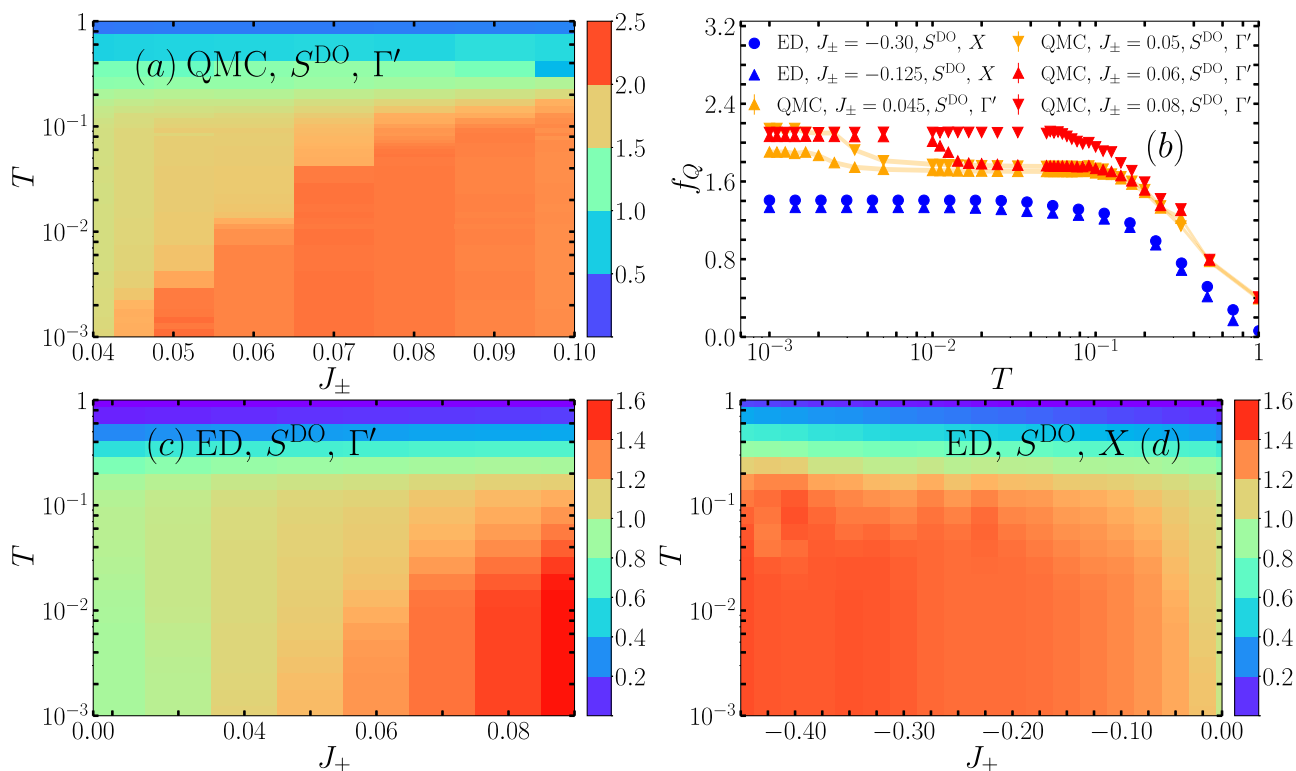
Fig. 3 | QFI in experimental coordinates for Cerium-based pyrochlore compounds. a presents a heat map of the QMC computed f_Q(S_r^{\text{DO}}, T) , with J_{\pm} ranging from 0.04 to 0.10. b is the line cut of (a) from J_{\pm} = 0.045 to 0.08. The crossover temperature scales from the paramagnetic phase to CSI at T \sim 1 and from
